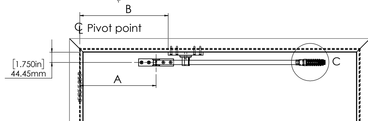
Elevation of door viewed from push side of door.
